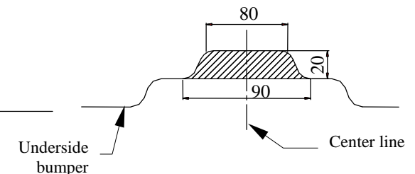
Fig. 3 Bumper cut out Mazda Tribute
